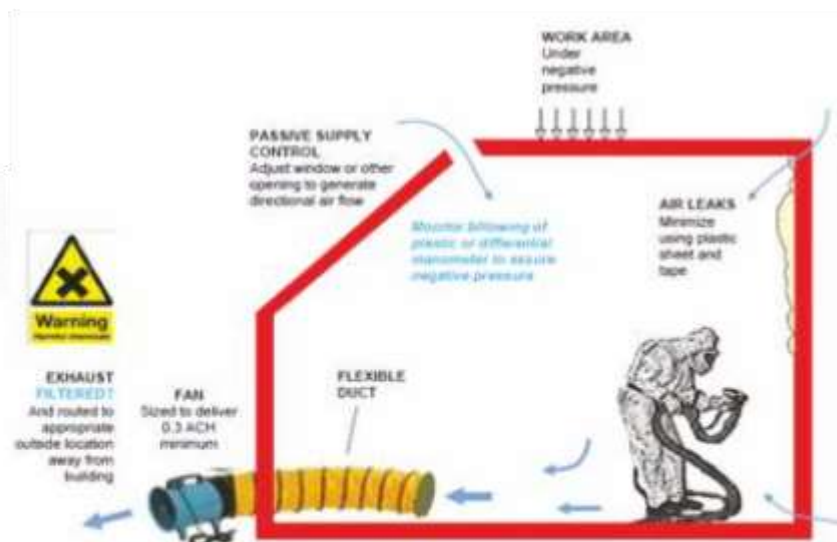
Figure 32 : An Ideal SPF operation
