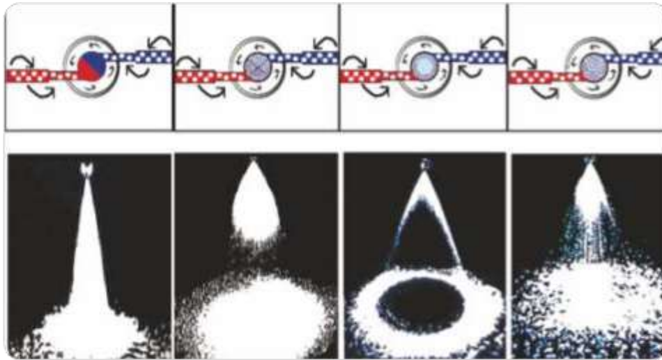
Figure 33 : Spray pattern vs temperature & pressure Potential Skin Injection Hazard
